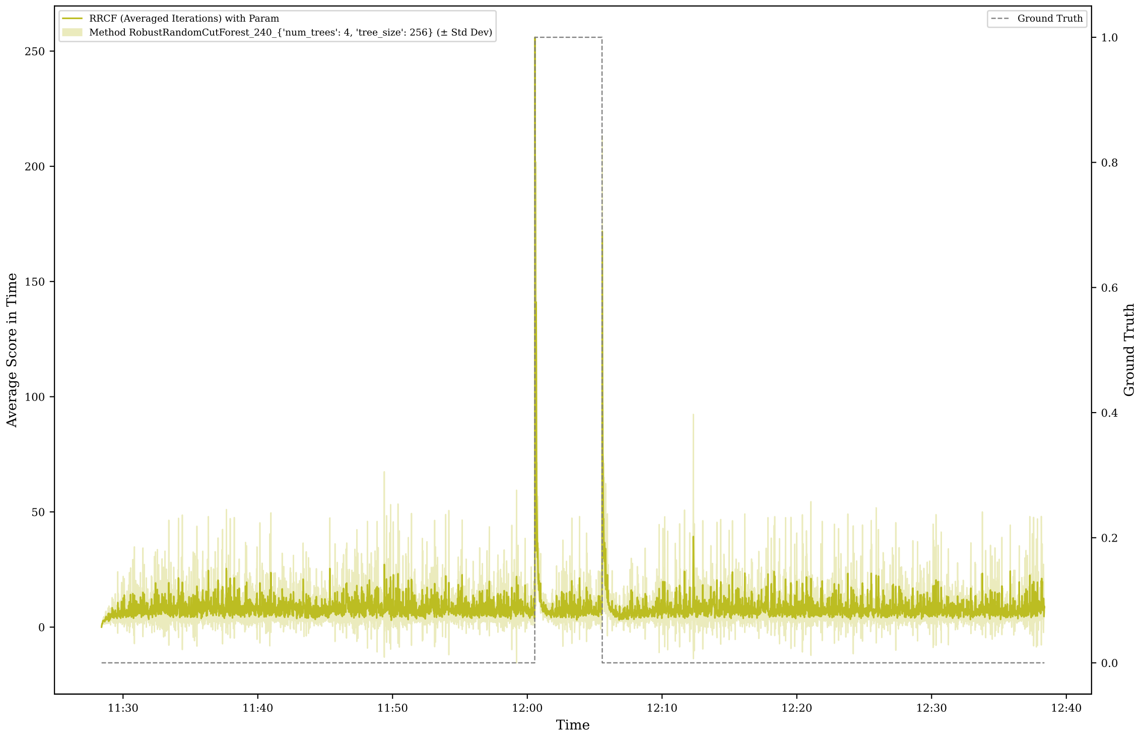
Method RRCF Score for Scenario A8
